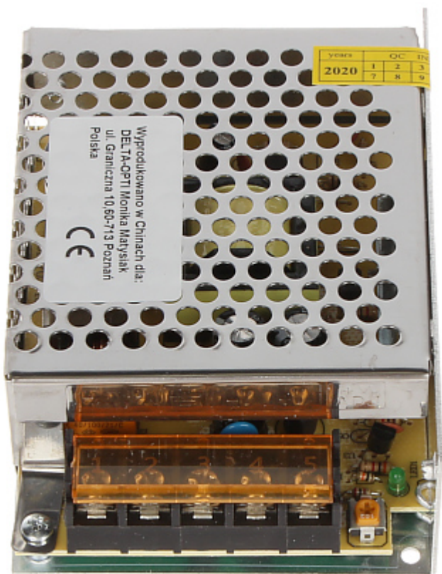
Adapter connectors:
