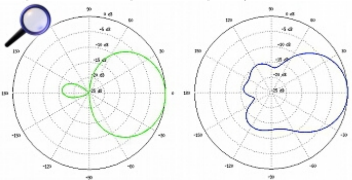
Polar pattern for vertical polarization (respectively horizontal and vertical plane):
