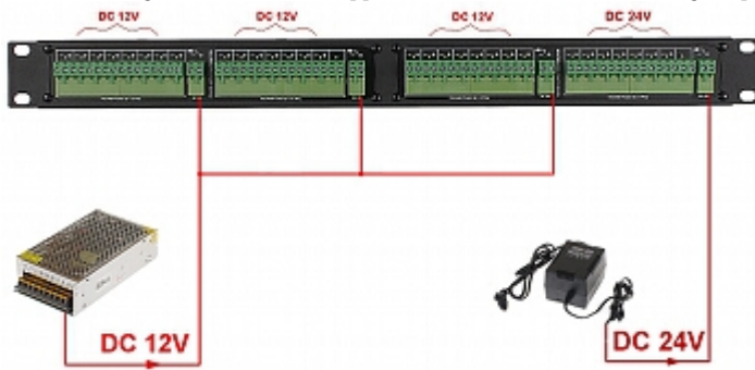
Schematic diagram of distributor application with two different voltages option
