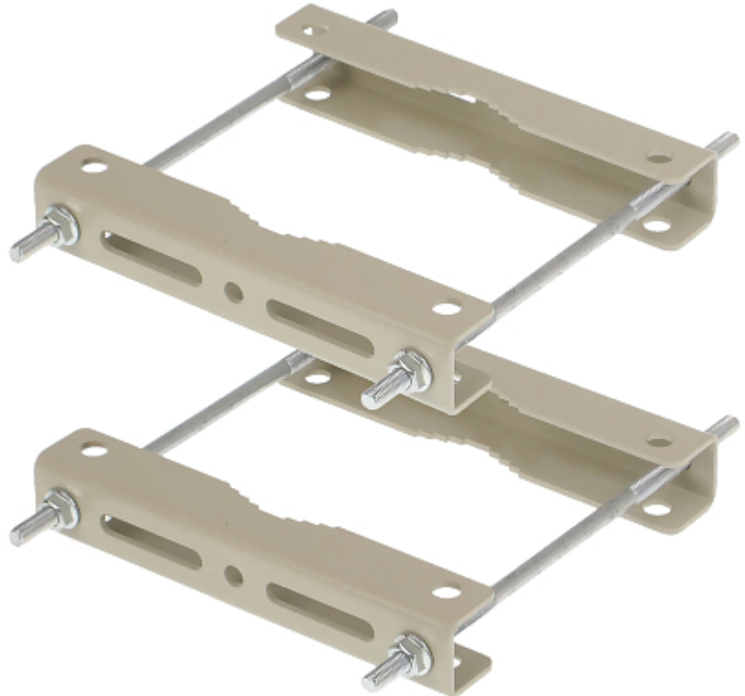
Clamp with reinforced profile. It enables mounting camera bracket to a pole.
