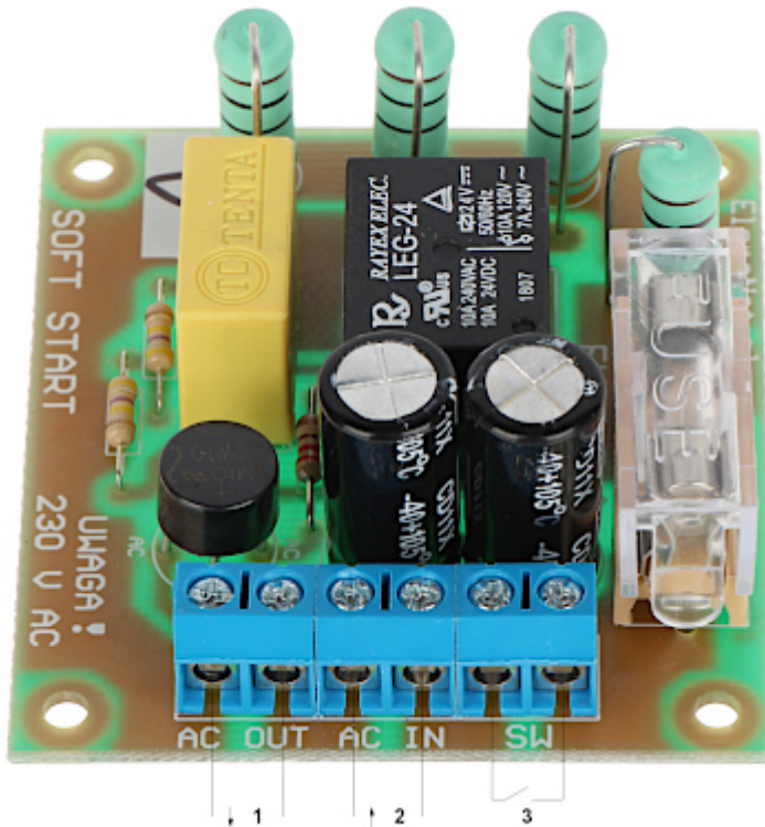
Connectors view
