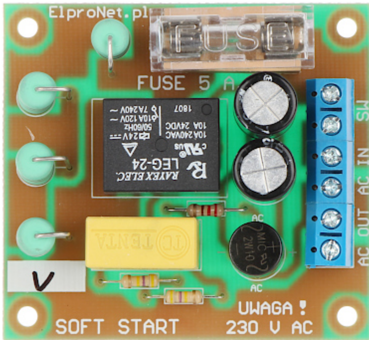
Connectors view
