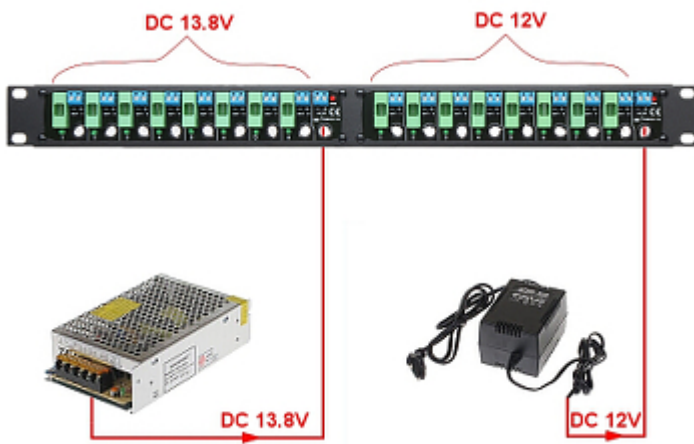
Schematic diagram of distributor application with two different voltages option:
