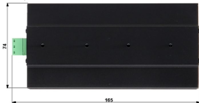
Mounting dimensions:
