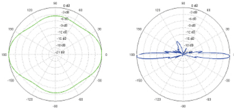
Polar pattern for horizontal polarization (respectively horizontal and vertical plane):
