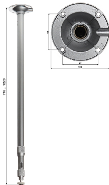
Bracket dimensions:
